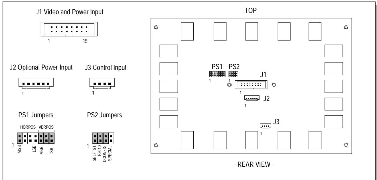
Fig 1. The input connectors and jumpers and their location on EL640.400-C2, -C3 and -CD3 display
