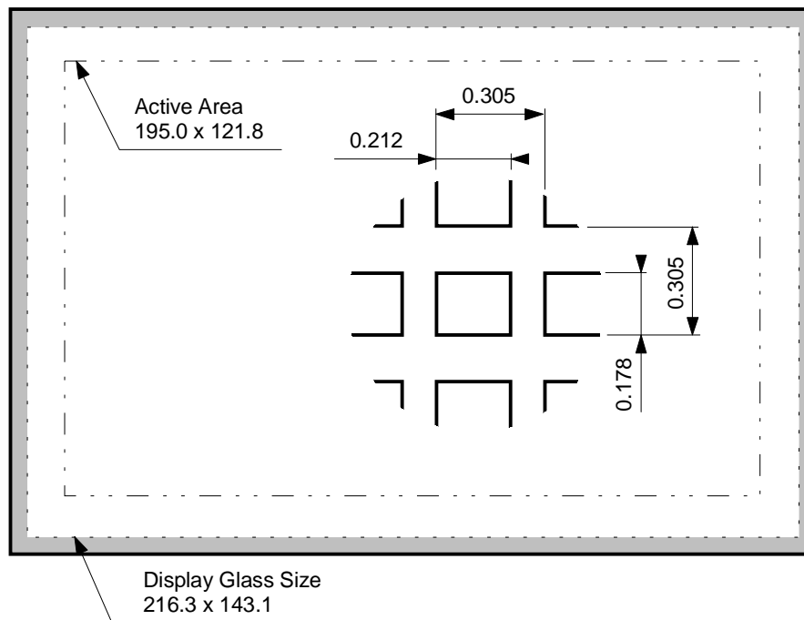
Fig. 2. EL640.400-C2, -C3 and CD3 display, viewing area characteristics
